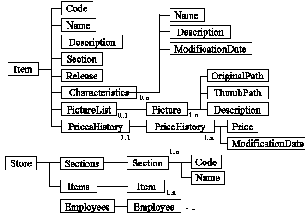
Figure 1: S_{\text{virtual\_store}} schema
