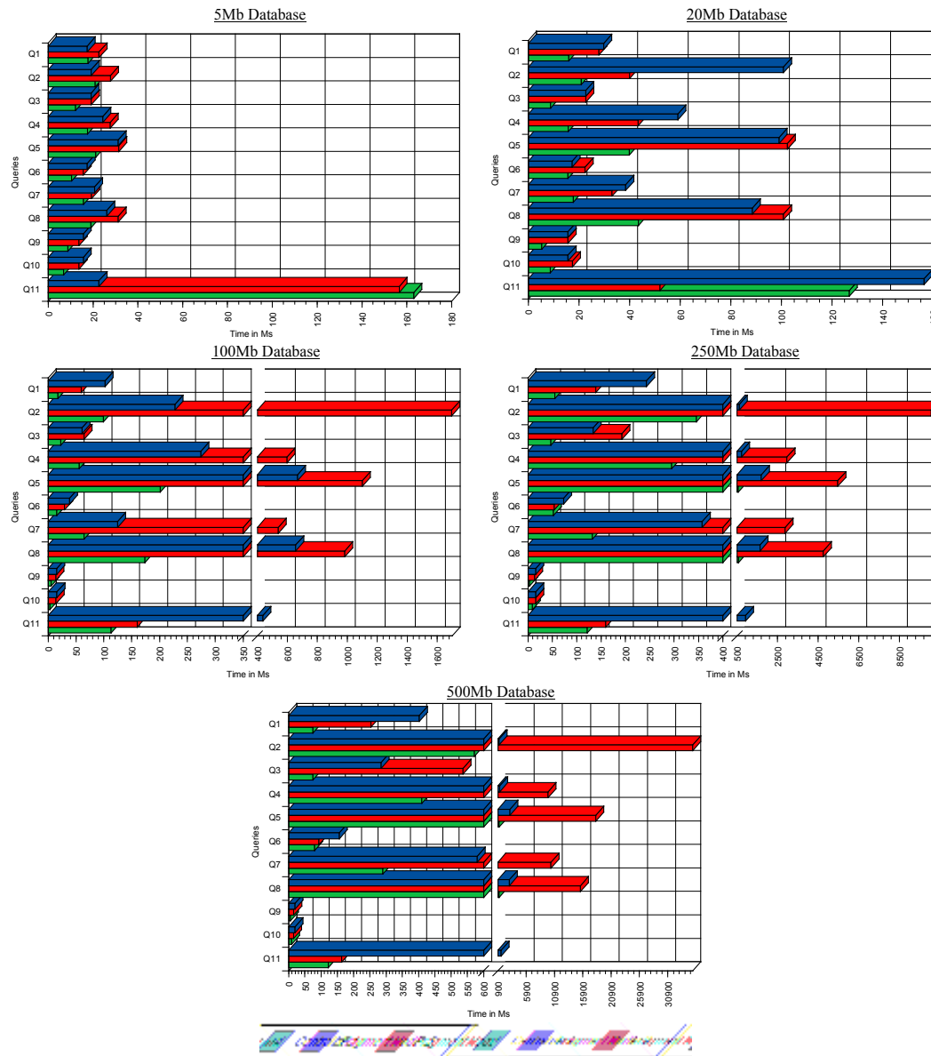
Figure 13: Experimental results for database Store_Hyb – hybrid fragmentation, without transmission times
